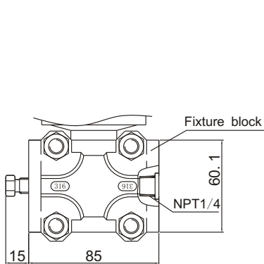
Process connecting type - leading pressure optional figure (P) - 1/4-18NPT taper pipe female thread
